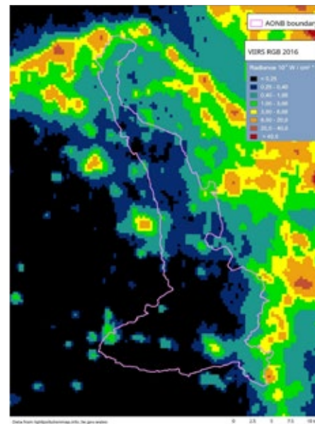
Figure 3: Radiance observed from space 2016
